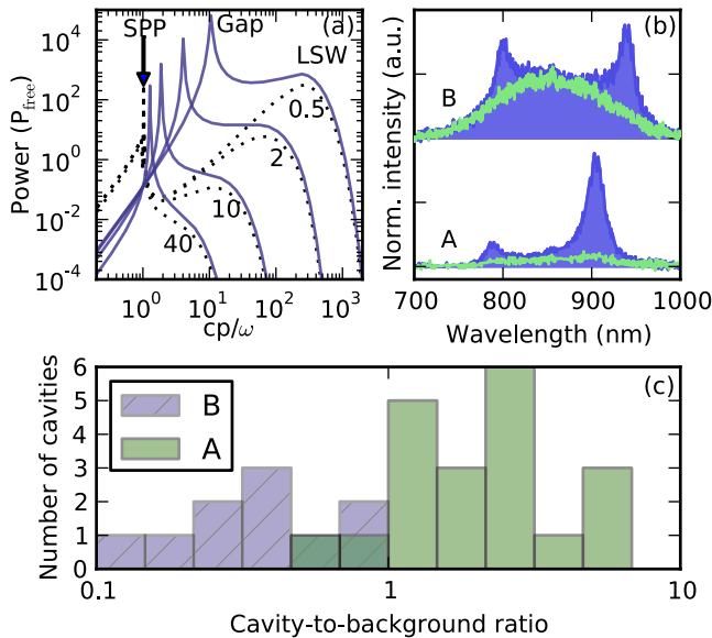
FIG. 3. (Color online) Resistance of gap mode to fluorescence quenching. (a) Calculations of emitted power at \hbar\omega=1.96 eV for a perpendicular dipole near a flat Ag surface (dotted) or between two parallel Ag surfaces (solid) as a function of the wave vector component parallel to the surface, p . Dipole-metal distance is indicated in nanometer; calculations are normalized to free-space dipole power spectrum, P_{\text{free}} . (b) Example fluorescence spectra from cavities with different NC-substrate spacings (total gap thickness of sample A, \sim 15 nm; B, \sim 40 nm) showing emission polarized parallel (filled curve) and perpendicular (line) to the NW axis. (c) Ratio of integrated cavity emission to integrated background emission for all devices measured from the two samples. [For the example spectra plotted in (b), this ratio is visually given by the area of the part of the filled curve above the green line divided by the area of the part below.] Note that the horizontal scale is logarithmic; values above one indicate that the cavity fluorescence is brighter than the background.
